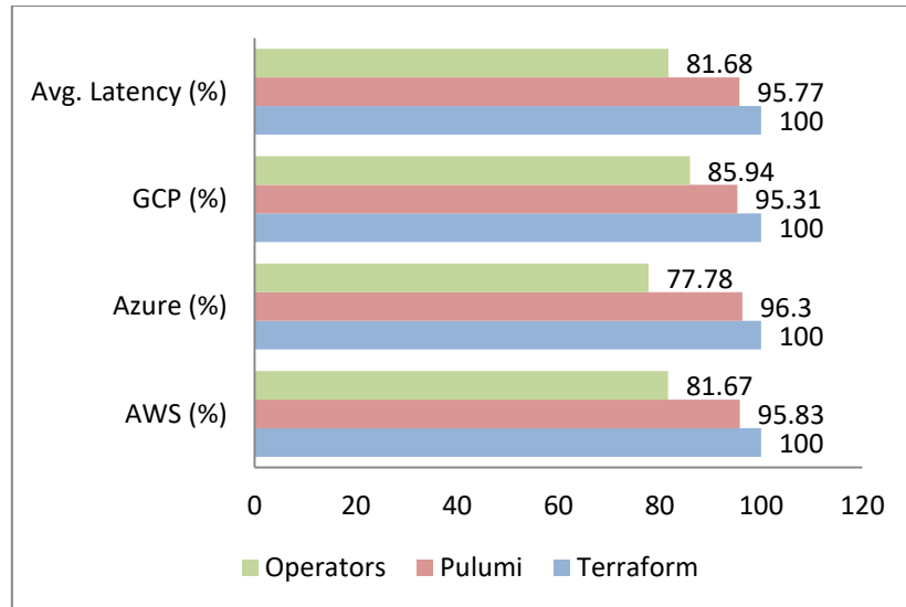
Fig 6: Graph representing Performance Comparison
